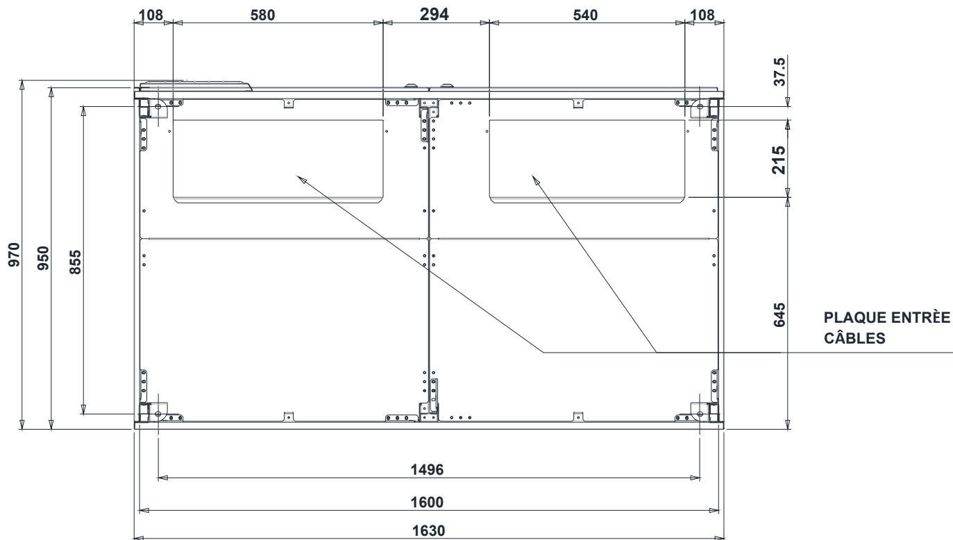
Illustration 3A – Plan de base KEOR HPE 600 kVA
