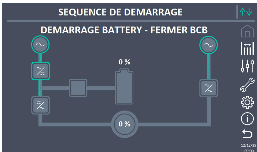
Illustration 16 – Battery start-up
