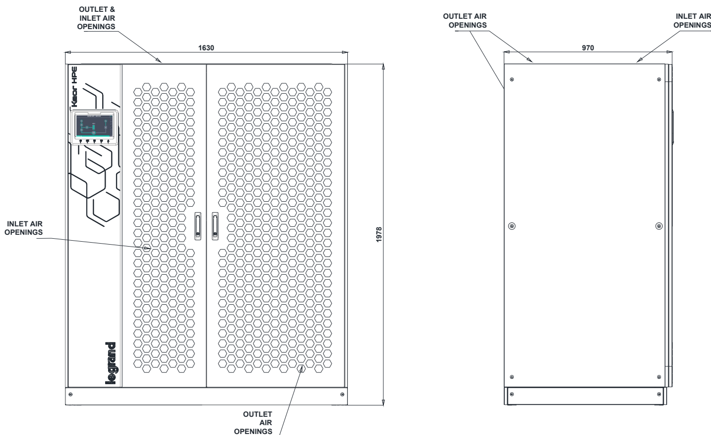
Picture 4A – Overall dimensions KEOR HPE 600 kVA
