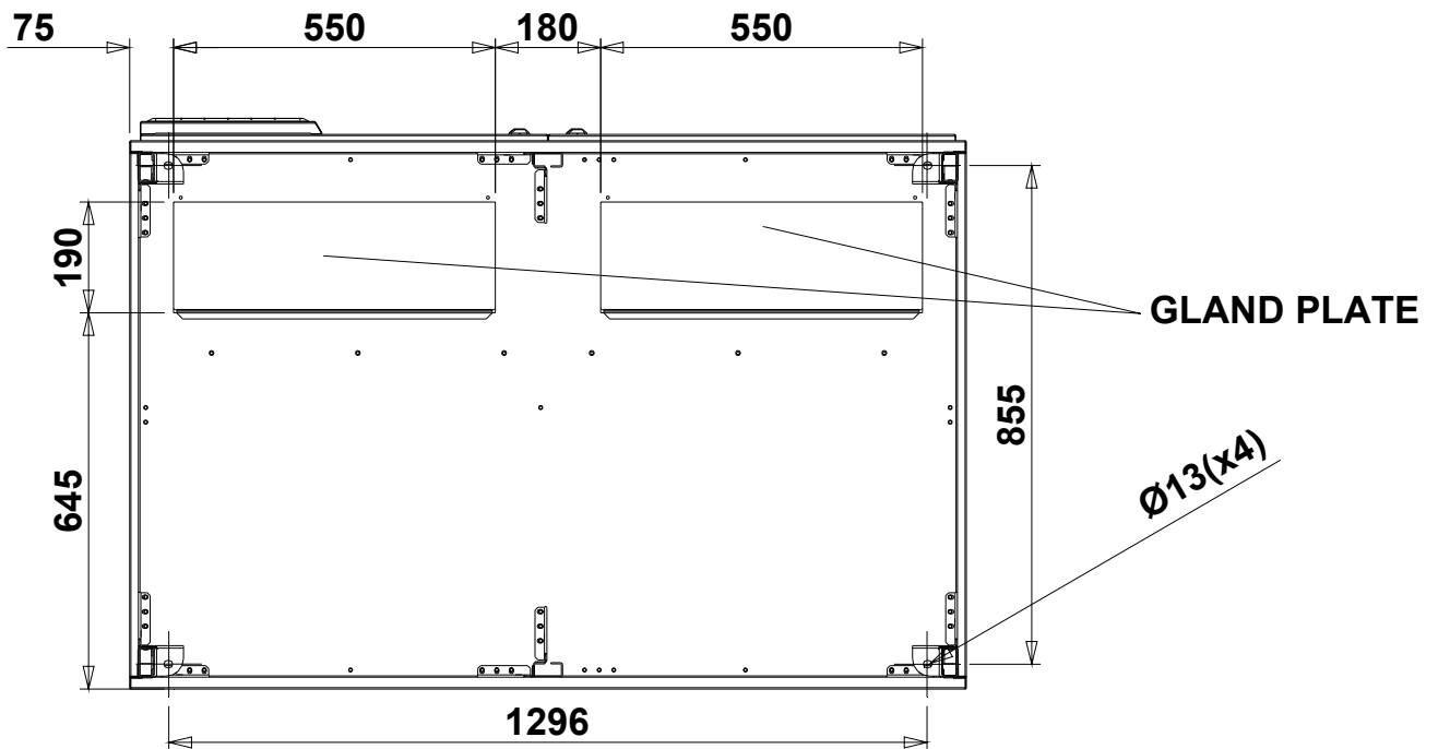
Picture 3 – Base plan KEOR HPE 400-500 kVA
