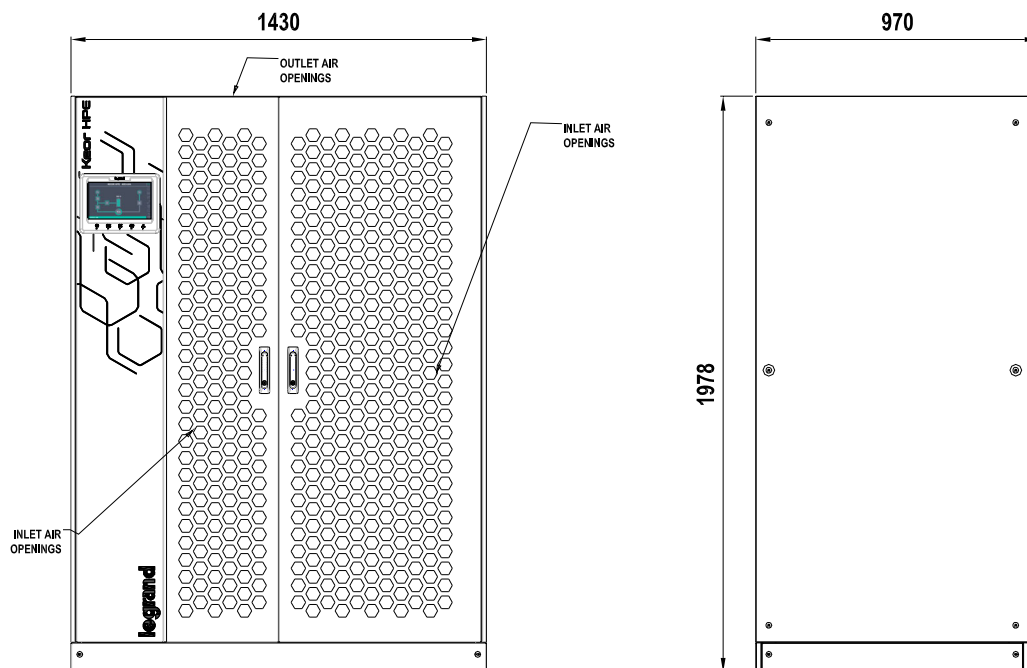
Picture 4 – Overall dimensions KEOR HPE 400-500 kVA
