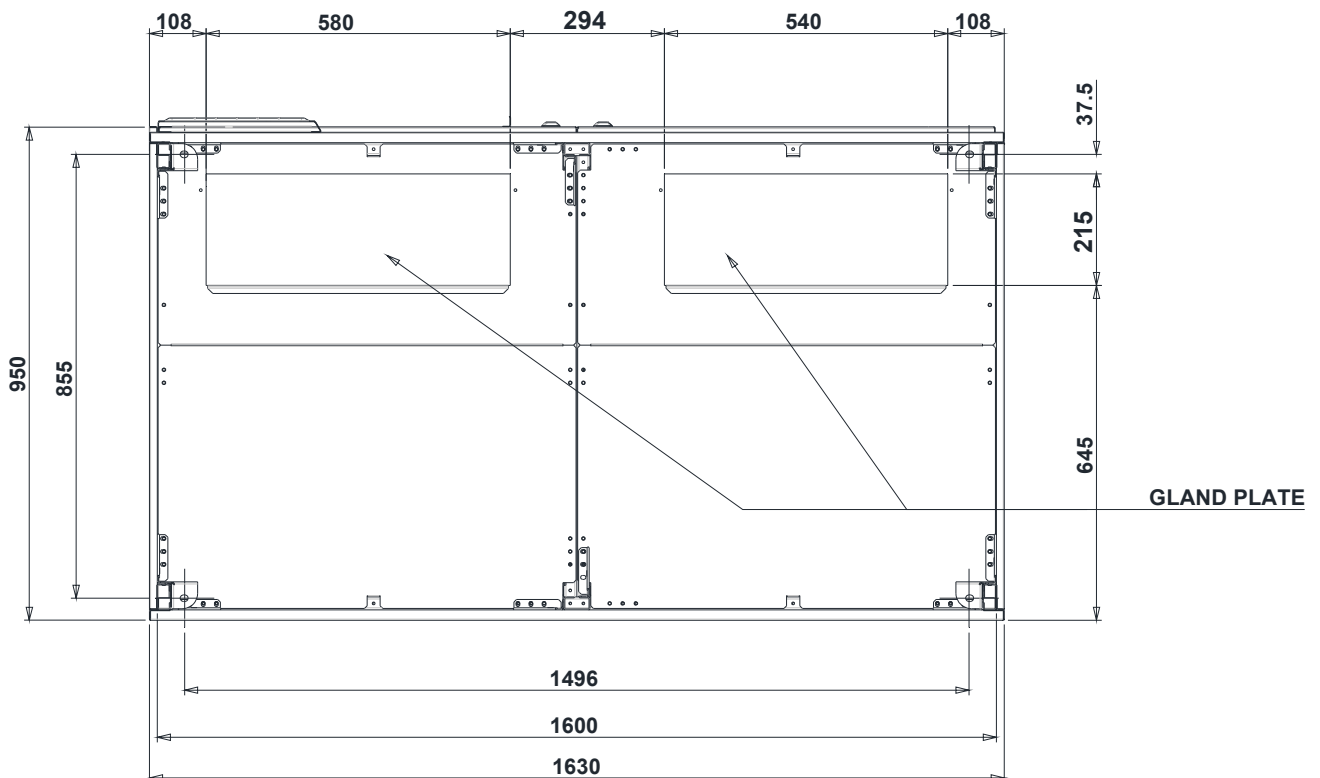
Picture 3A – Base plan KEOR HPE 600 kVA
