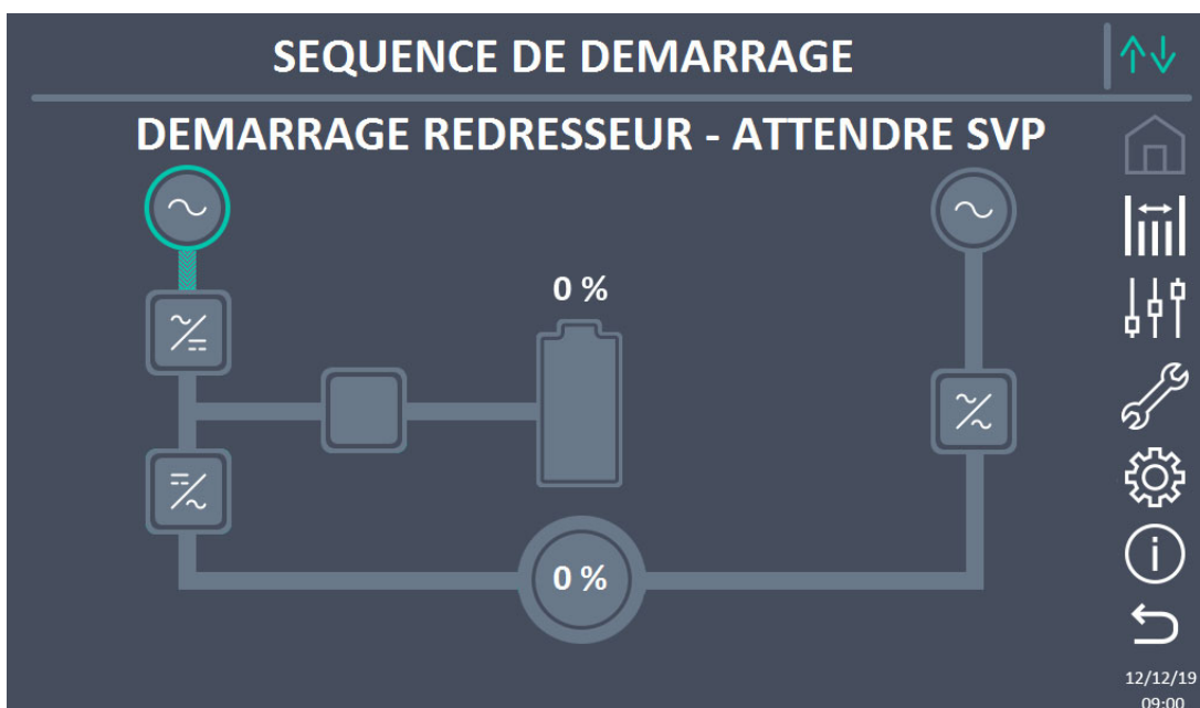
Illustration 13 – Rectifier start-up
