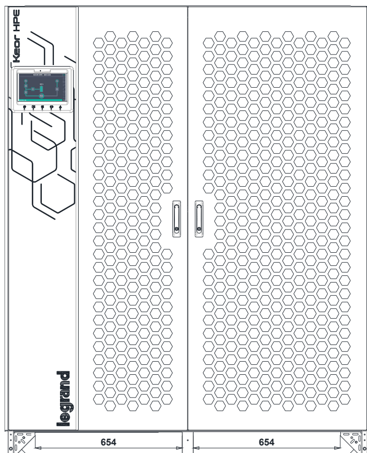
Picture 2A – Handling of the KEOR HPE UPS 600 kVA
