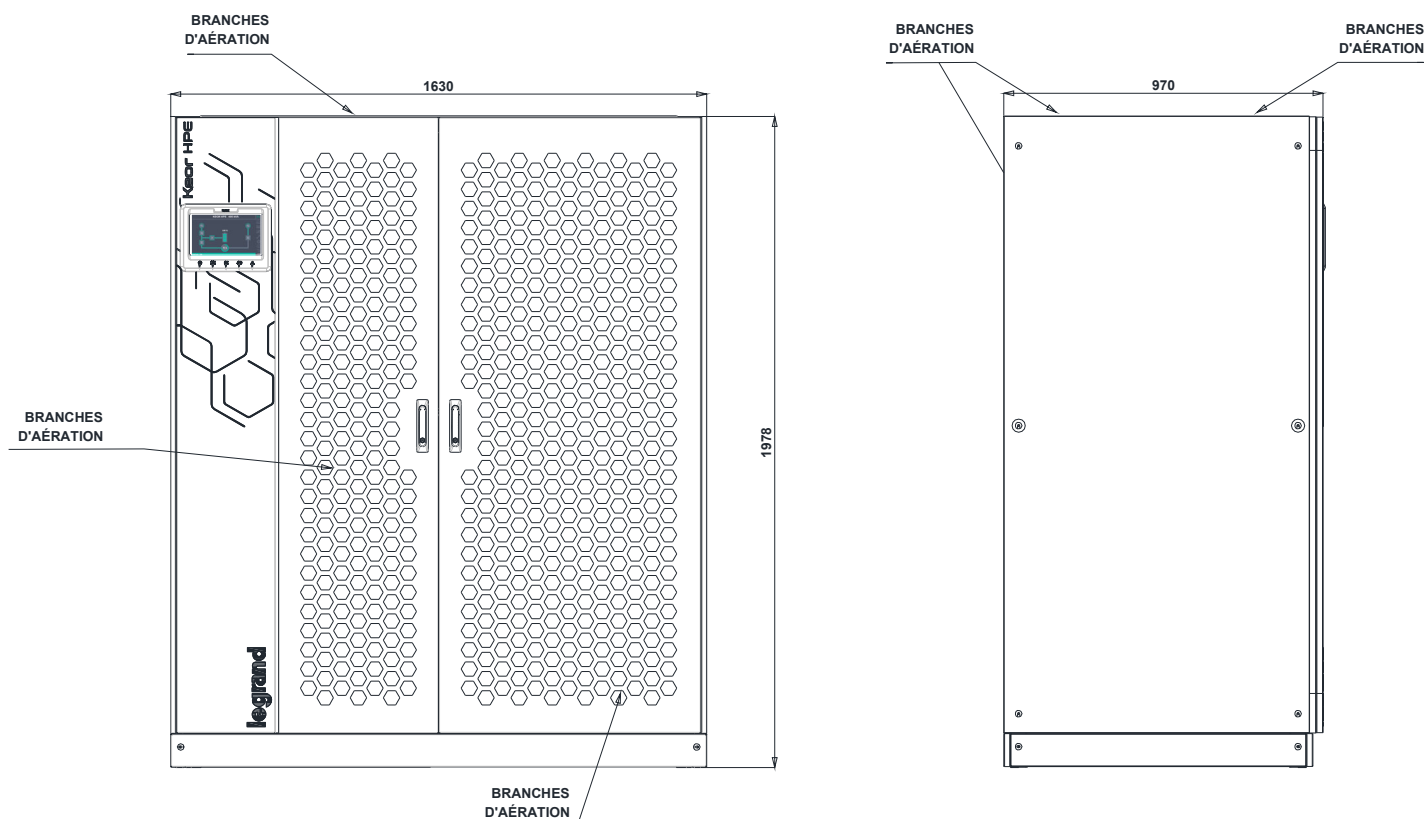
Illustration 4A – Dimensions globales KEOR HPE 600kVA
