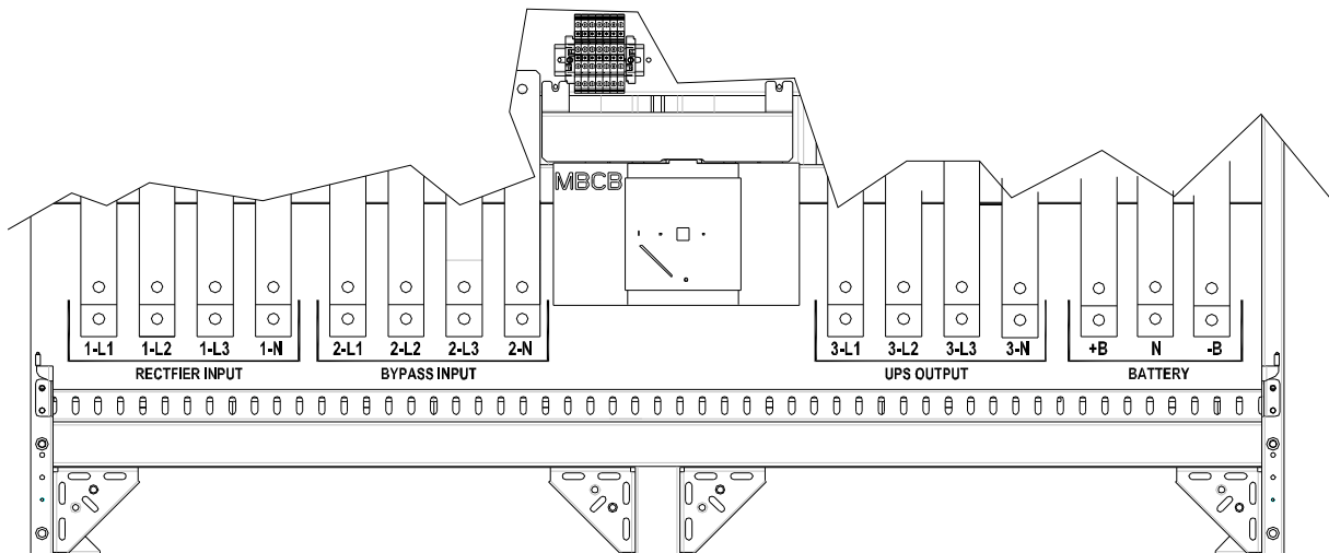
Picture 8A – Terminal board KEOR HPE 400-500 kVA
