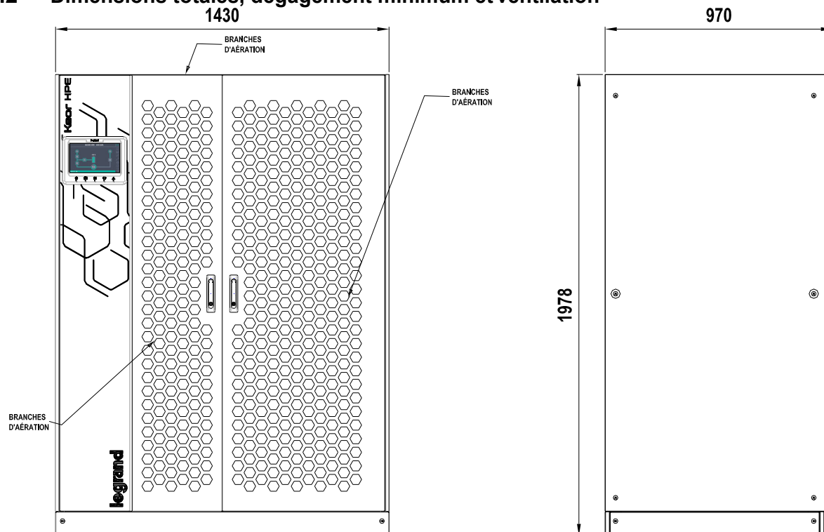
Illustration 4 – Dimensions globales KEOR HPE 400-500kVA
