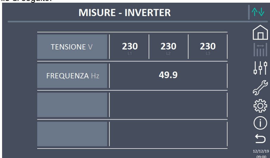
Figura 10 – Misure Inverter
