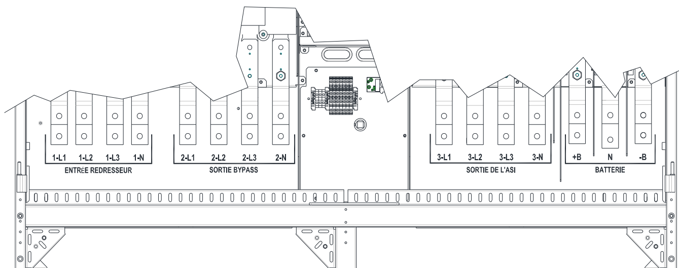
Illustration 8B – Borniers KEOR HPE 600 kVA
