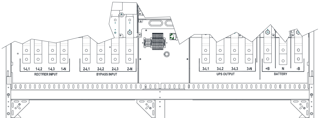
Picture 8B – Terminal board KEOR HPE 600 kVA
