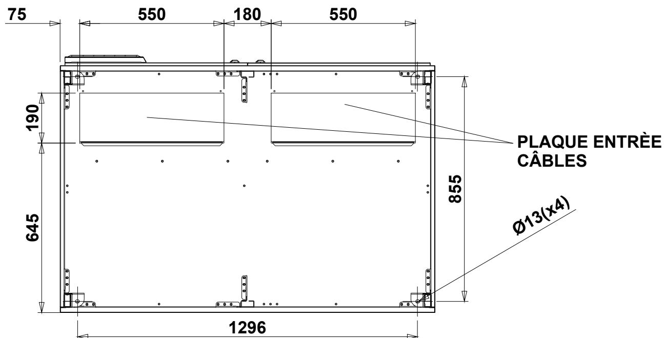
Illustration 3 – Plan de base KEOR HPE 400-500 kVA
