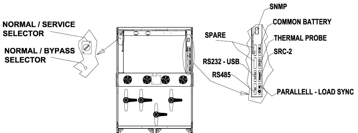
Picture 10 – Position of the serial interfaces of KEOR HPE 400-500 kVA
