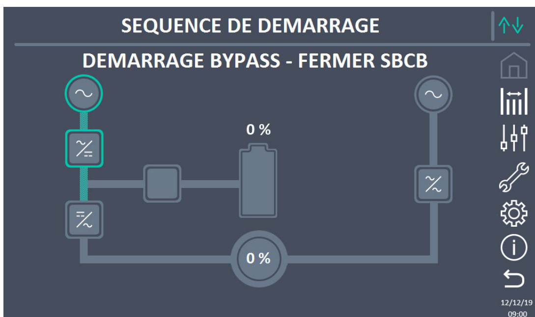
Illustration 15 – Bypass start-up
