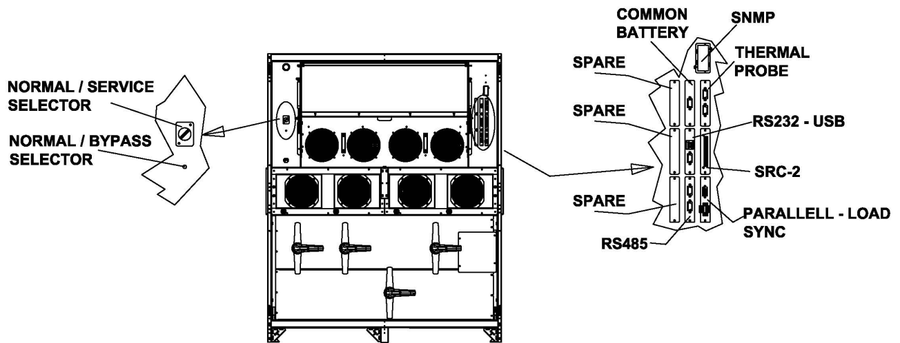
Picture 10A – Position of the serial interfaces of KEOR HPE 600 kVA
