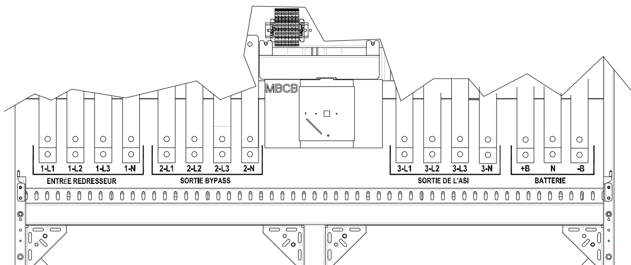
Illustration 8A – Borniers KEOR HPE 400-500 kVA
