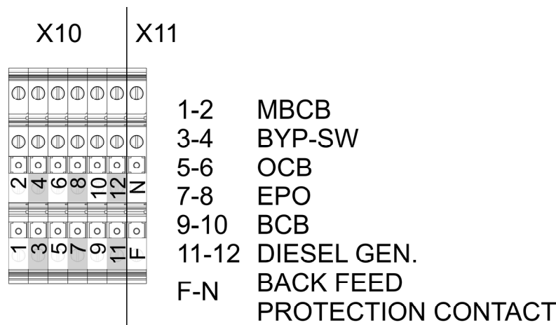
Picture 9 – Auxiliary terminals of KEOR HPE 400-500 kVA
