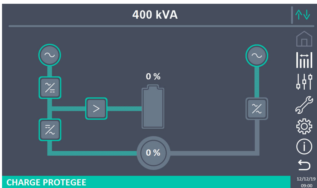
Illustration 18 – Start-up end
