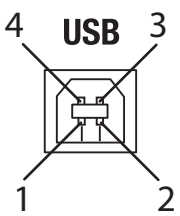
USB CONNECTOR:
