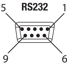
RS232 CONNECTOR:
