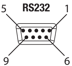
RS232 CONNECTOR:
