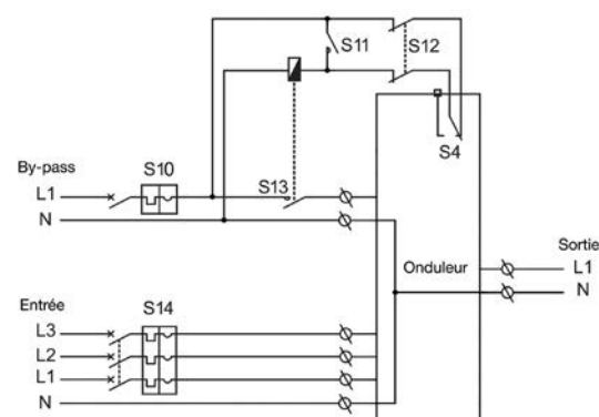
Configuration Triphasé/Monophasé
