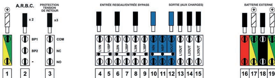
Trimod MCS 10 - 15 - 20
