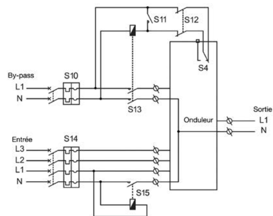
Configuration Triphasé/Monophasé
