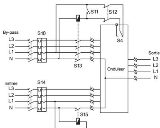
Configuration Triphasé/Triphasé
