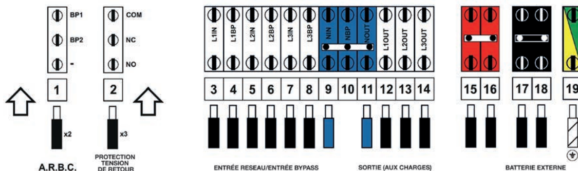
Trimod MCS 80
