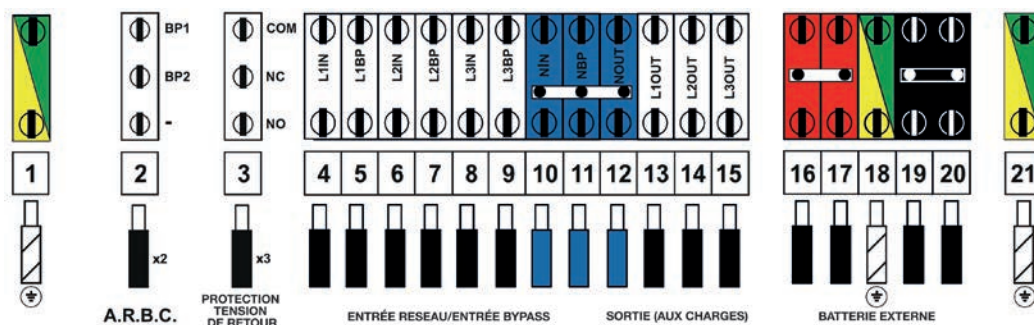
Trimod MCS 30
