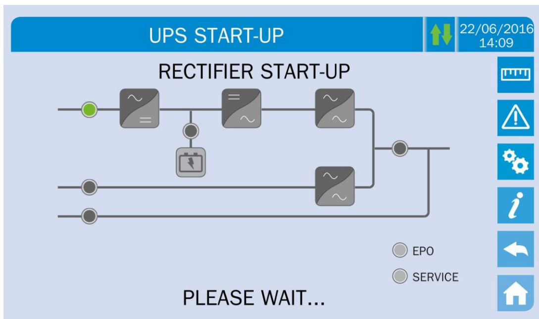
Illustration 11 – Rectifier start-up
