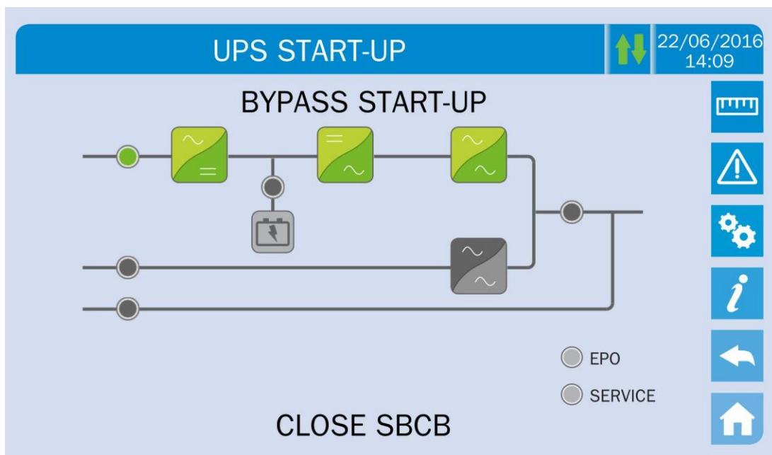
Illustration 13 – Bypass start-up
