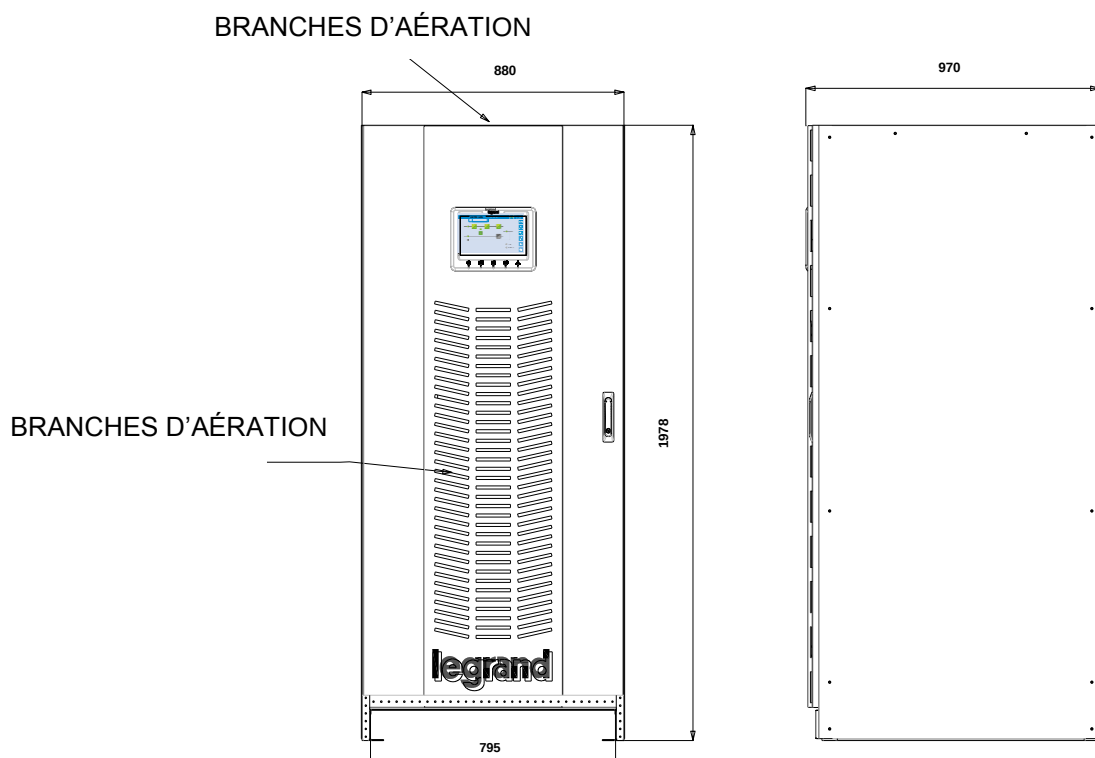
Illustration 4 – Dimensions globales
