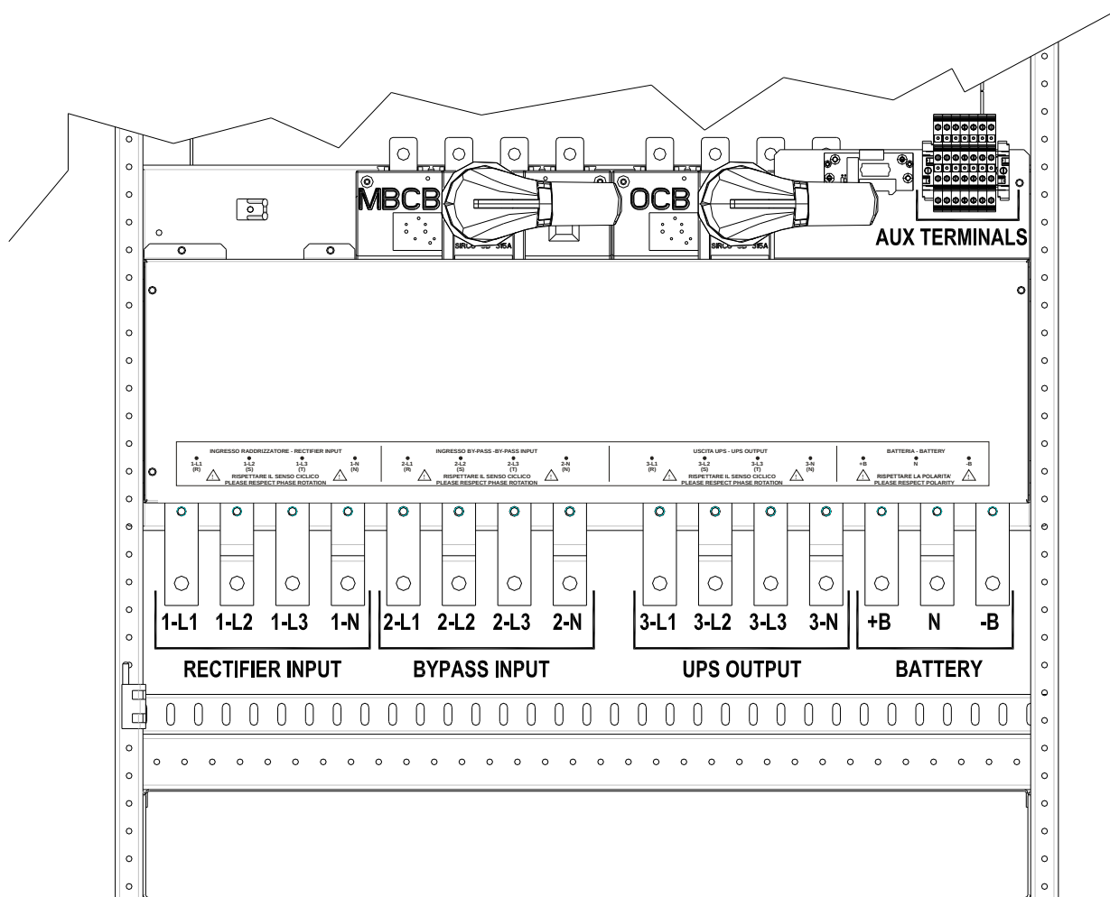
Picture 6A – Terminal board KEOR HPE 300 kVA
