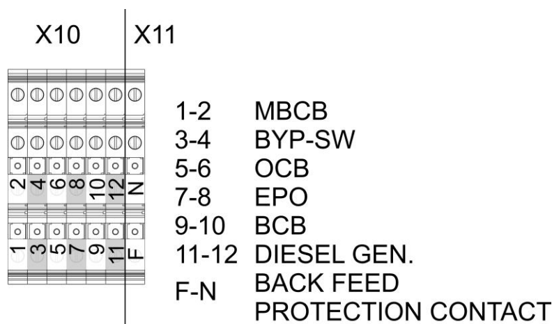
Picture 7 – Auxiliary terminals of KEOR HPE 200-250-300 kVA
