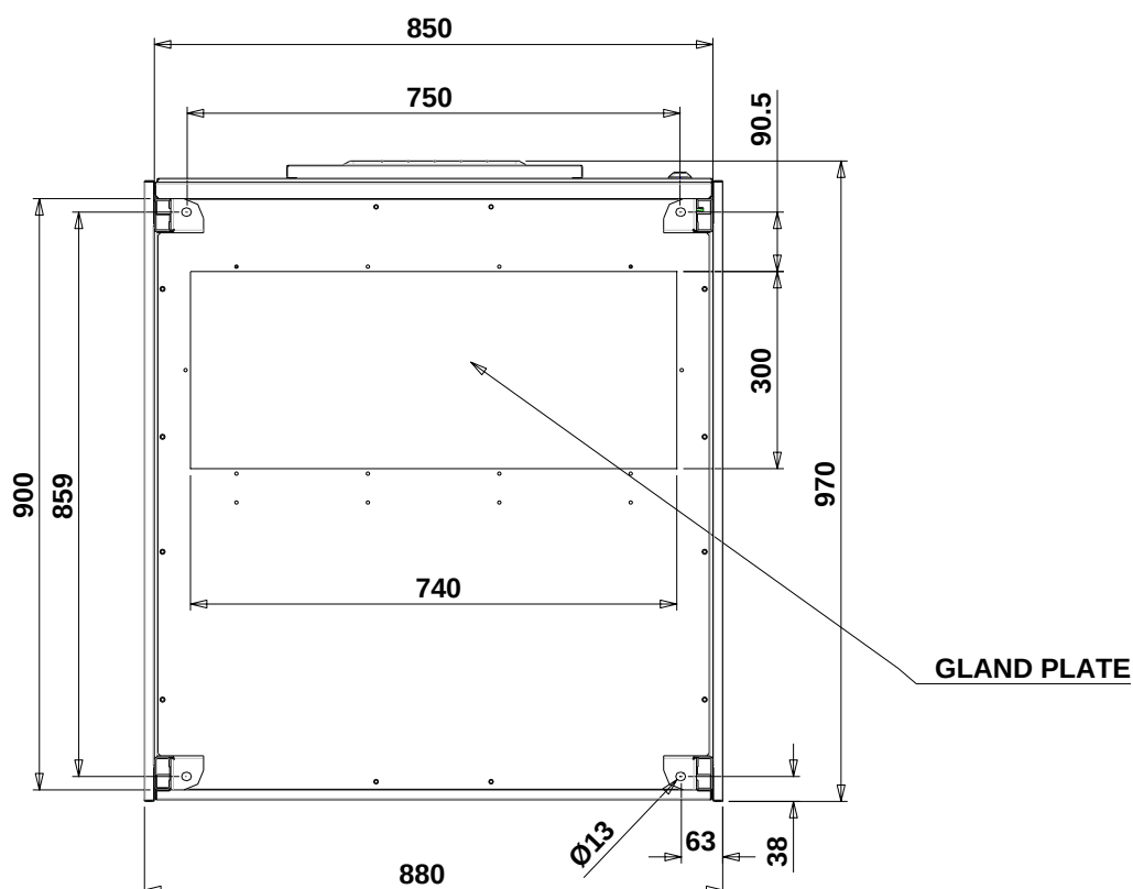
Picture 3 – Base plan
