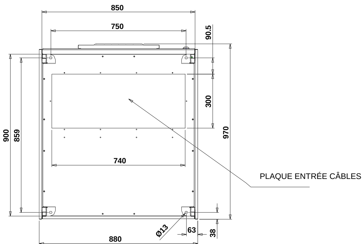
Illustration 3 – Plan de base
