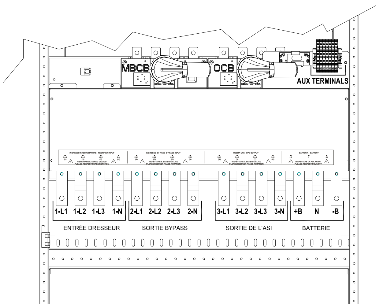
Illustration 6A – Borniers KEOR HPE 300 kVA
