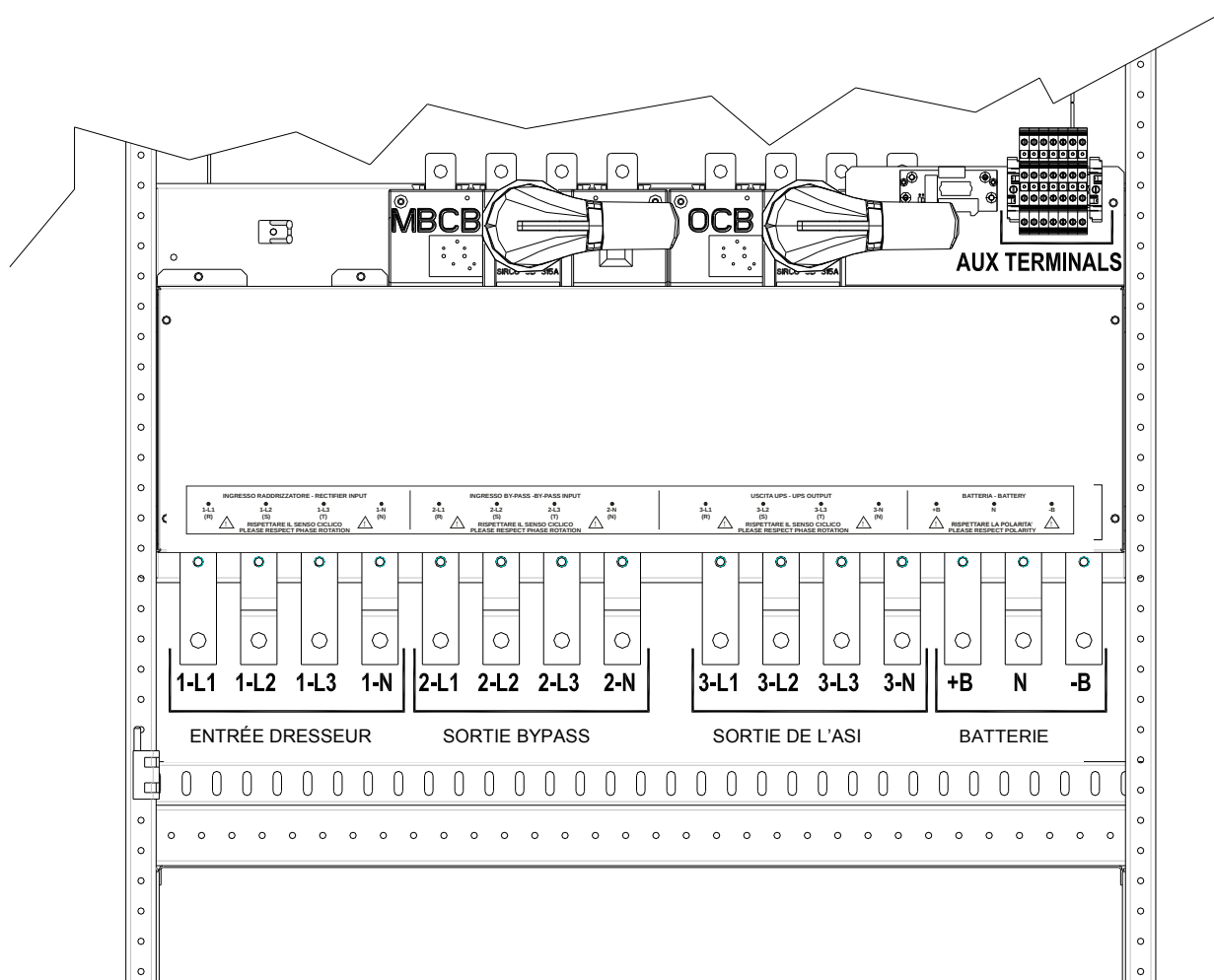
Illustration 6 – Borniers KEOR HPE 200-250 kVA
