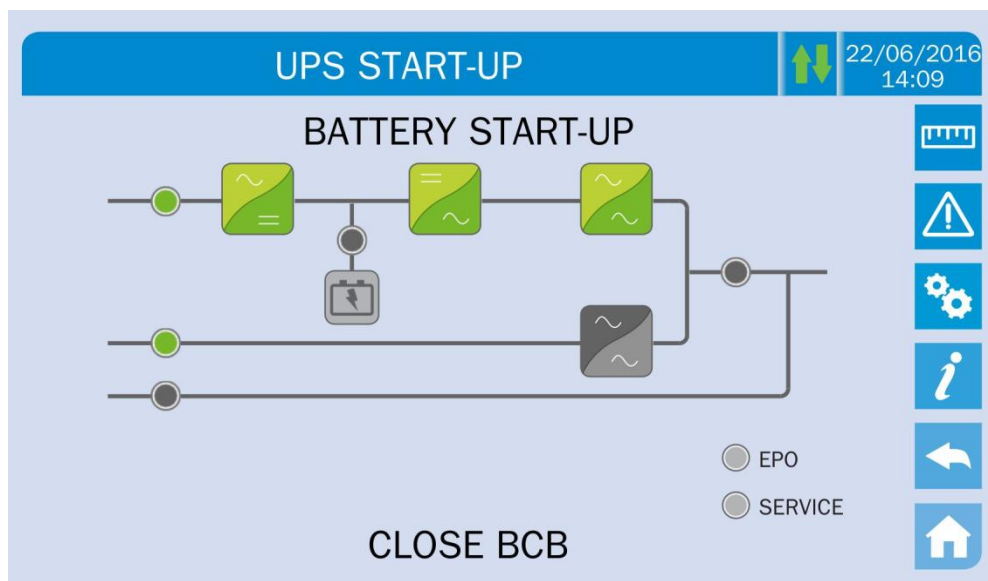
Illustration 14 – Battery start-up
