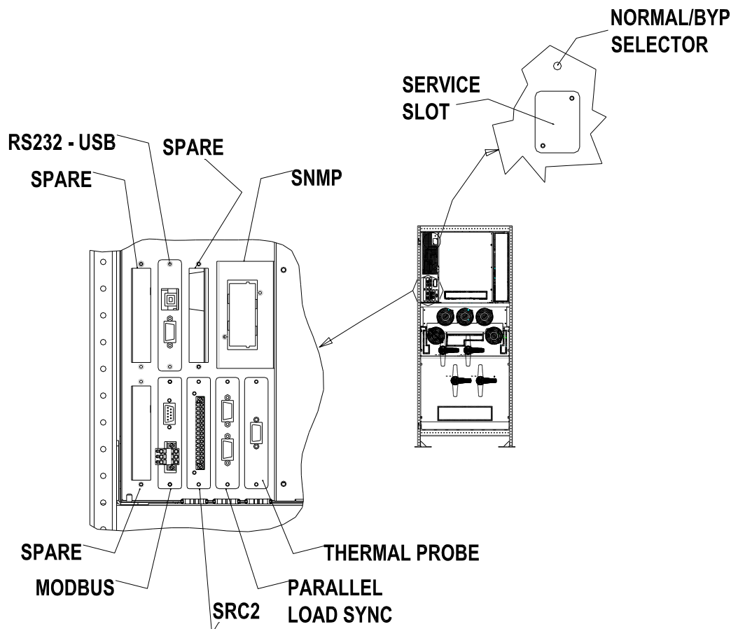
Picture 8 – Position of the serial interfaces of KEOR HPE 200-250-300 kVA
