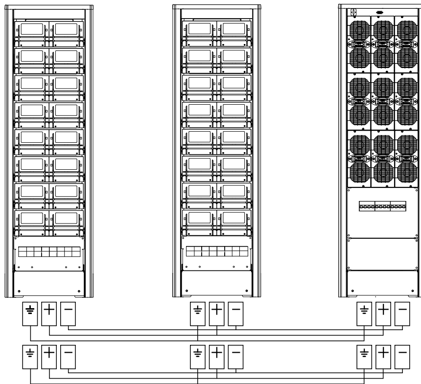
UPS Trimod® 40/60
